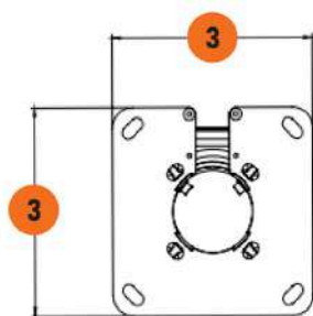
Footprint of standard installation flange
